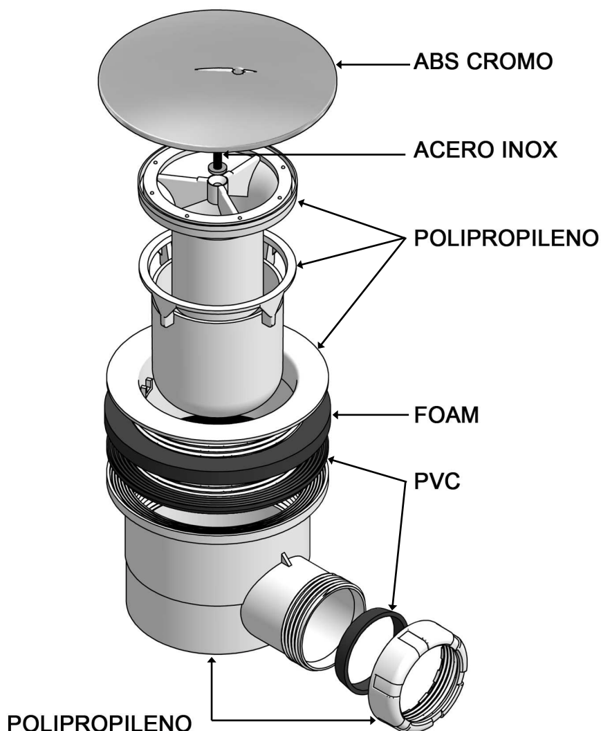
DESPIECE
